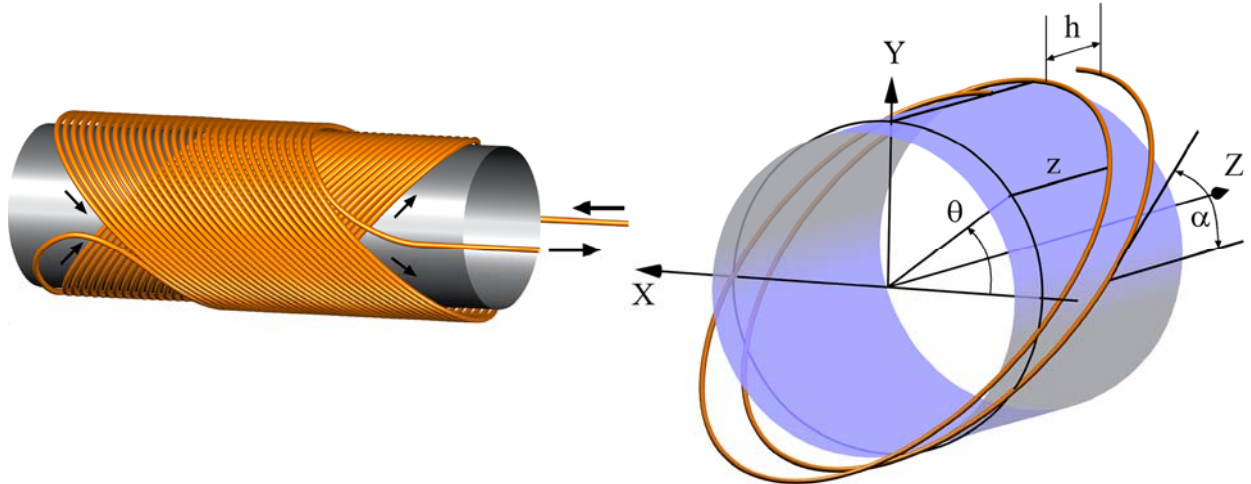
Figure 1. (Left) Layout of double helix winding. The axial field components of the 2 layers cancel each other and the total transverse field is enhanced. (Right) For the case of a dipole, the z coordinate of the conductor path is given by z(\Theta) = h \Theta / 2\pi + A_0 \sin \Theta with A_0 = a / \tan \alpha where a is the radius of the coil aperture, \alpha is the tilt angle of the winding with respect to the horizontal axis, and h is the helical advance per turn.
