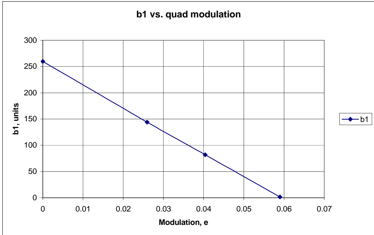
Figure 6. Units of quadrupole produced in the bent coils of Figure 5 (without iron) as a function of the quadrupole modulation factor ( \epsilon_2 ) of the coil.
