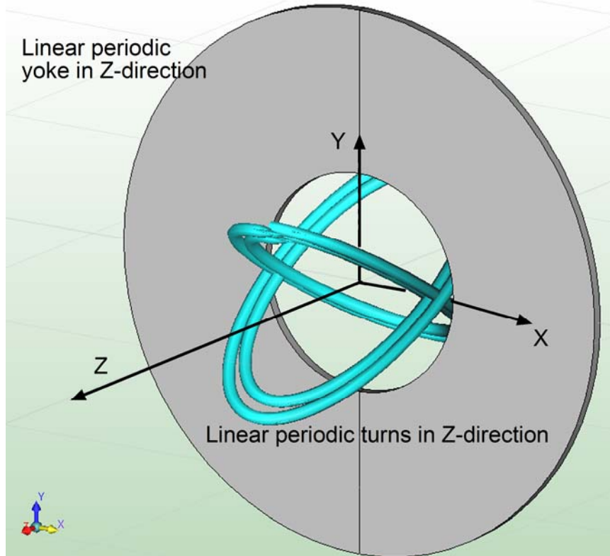
Figure 7. Linear periodic model of a 4-layer double-helix coil in an iron yoke.
