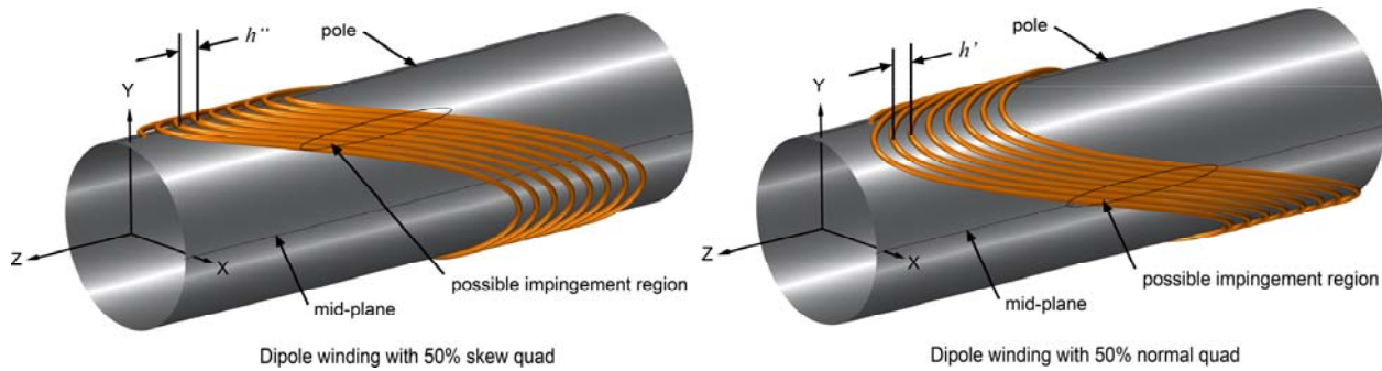
Figure 4. Dipole windings with 50% skew and normal quad amplitudes.
