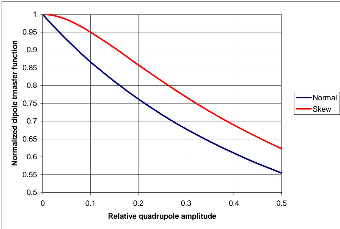
Figure 3. The dipole transfer function decreases with the amount of quadrupole amplitude because of the conductor impingement limitation. The difference between the normal and skew quadrupole come from the geometrical effect of the winding.
