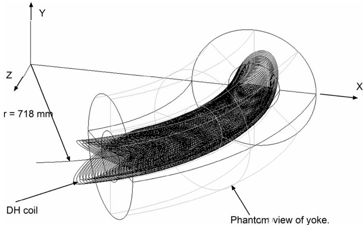
Figure 5. Diagram of a proposed 4-layer double-helix coil used in a 180° beam channel bend.
