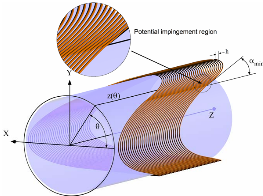
Figure 2. Potential impingement region of a double-helix winding for a quadrupole coil example. With an effective conductor width, d , the axial turn spacing has to be h \geq \frac{d}{\sin \alpha} in order to prevent the conductors from overlapping where the tilt angle, \alpha , is a minimum. This occurs at \theta = 45^\circ in a quadrupole and at the mid-plane ( \theta = 0^\circ ) in a dipole.
